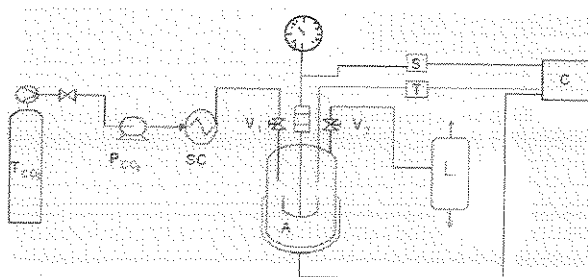
Figure 1 The experimental apparatus: A, vessel with external heater; C, Temperature and magnetic stirrer PID controller; T, thermocouple; S, magnetic stirrer; L, liquid separator. P CO 2 , carbon dioxide pump; SC, cooler system with Peltier effect; T CO 2 , carbon dioxide tank; V 1 , inlet globe valve; V 2 , outlet globe valve.
